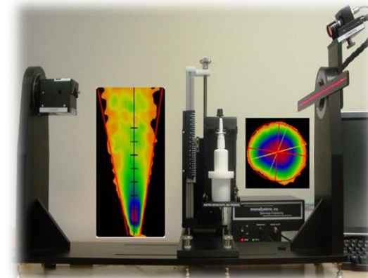
ISI-5000 Aerosol Drug Spray Analyzer
